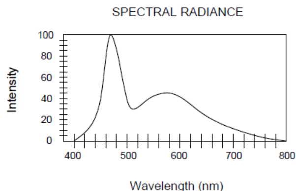
Fig.5 Luminous Spectrum(Ta=25°C)
